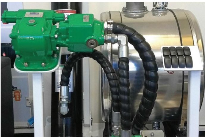
PTO & Pumps
