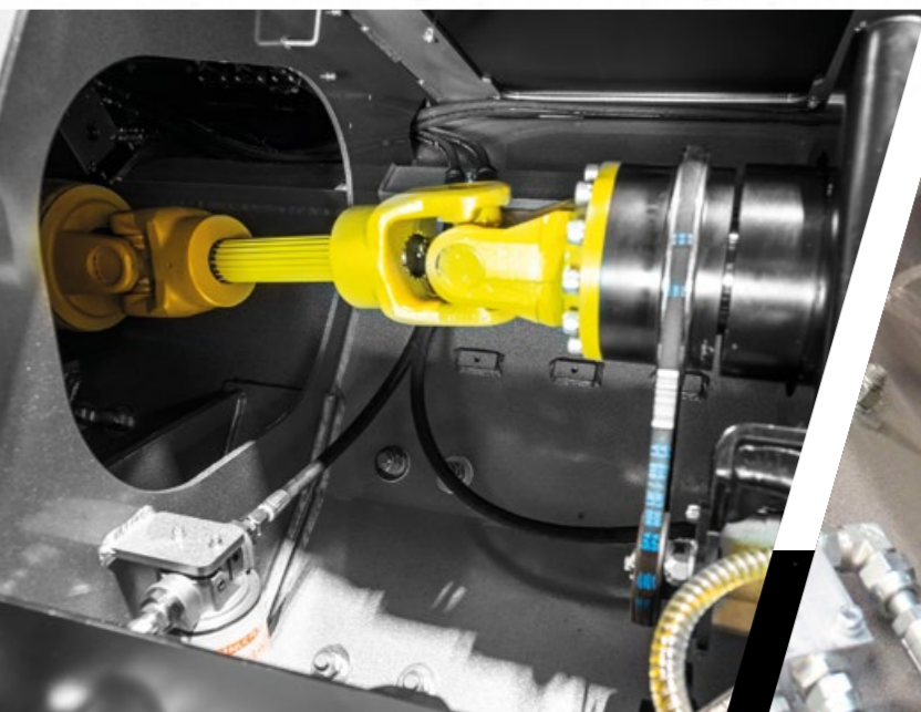
FRICTION CLUTCH
