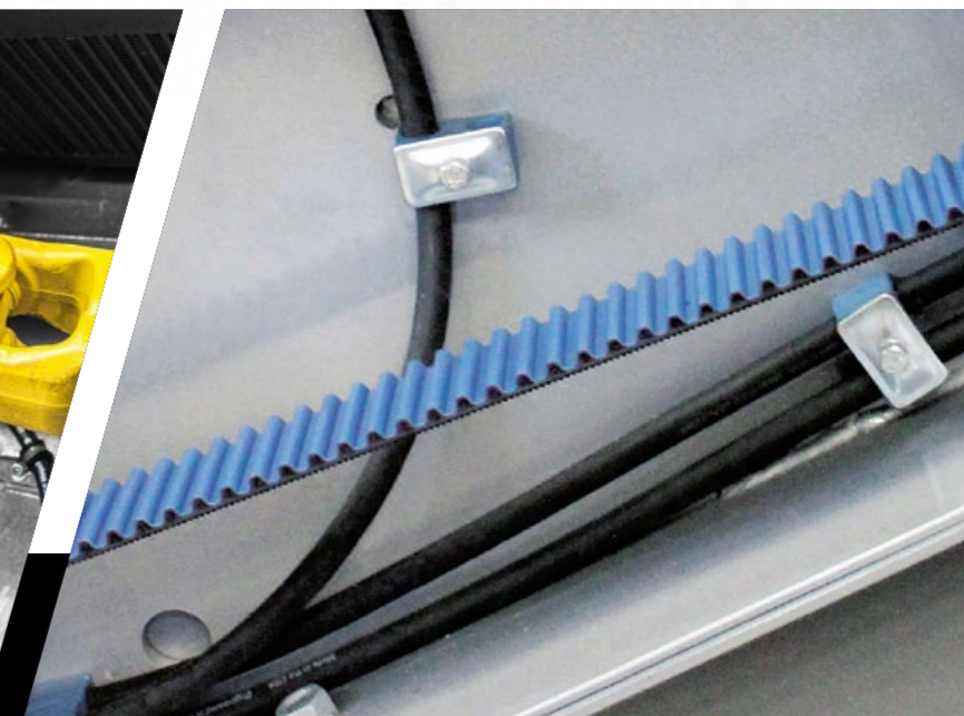
POLY-CHAIN® BELTS
